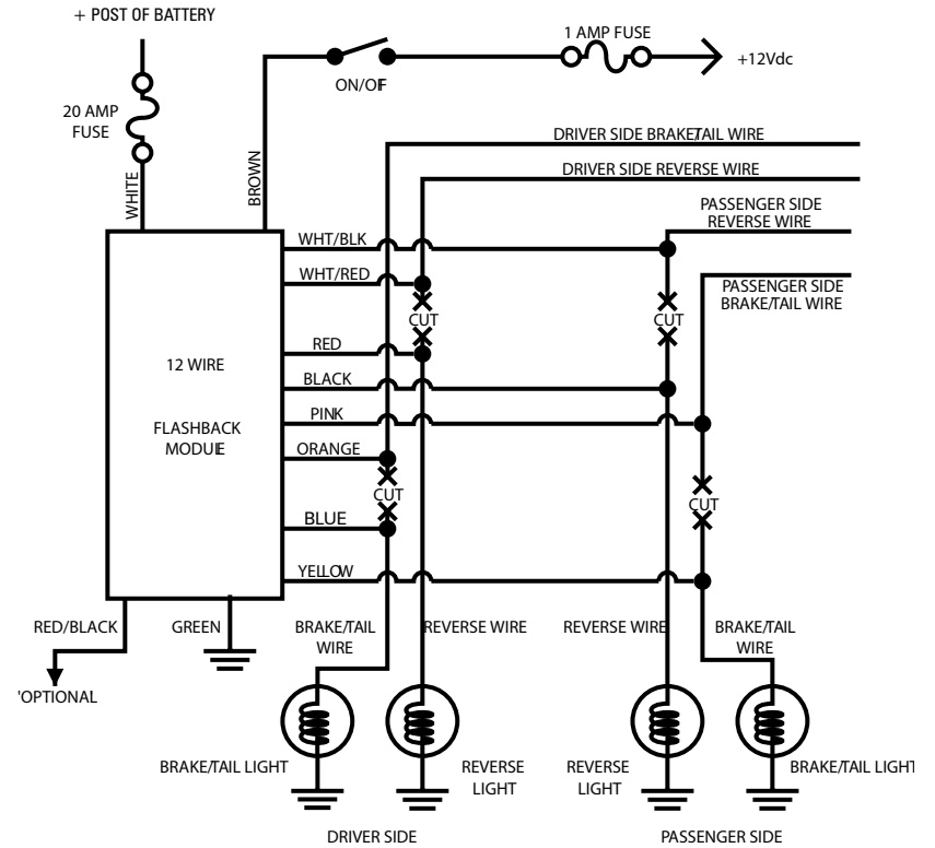
Diagram for use without Plugs
