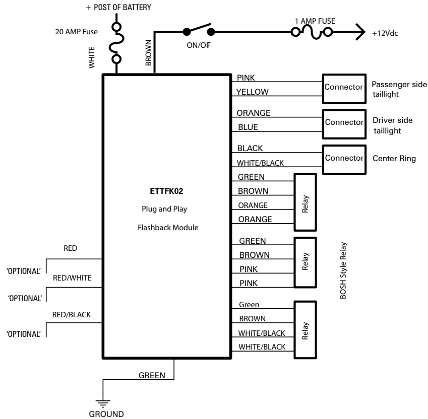
Diagram for use with Plugs
