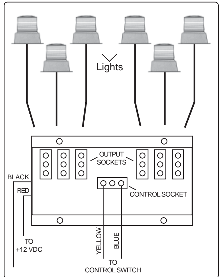
Wiring Diagram
