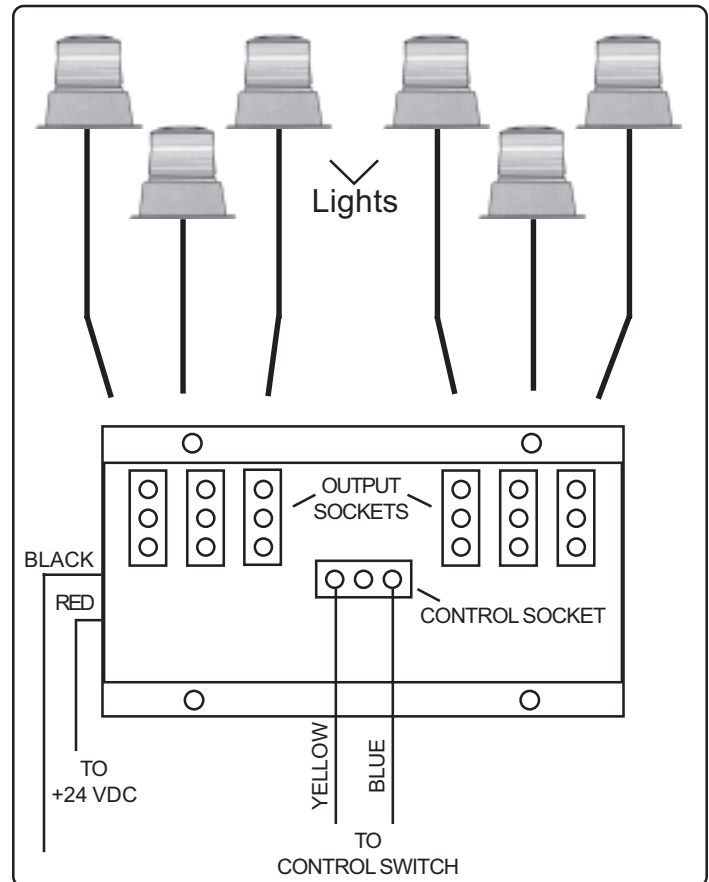
Wiring Diagram
