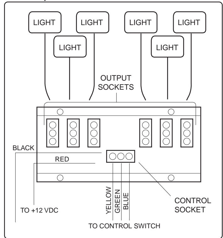
Wiring Diagram
